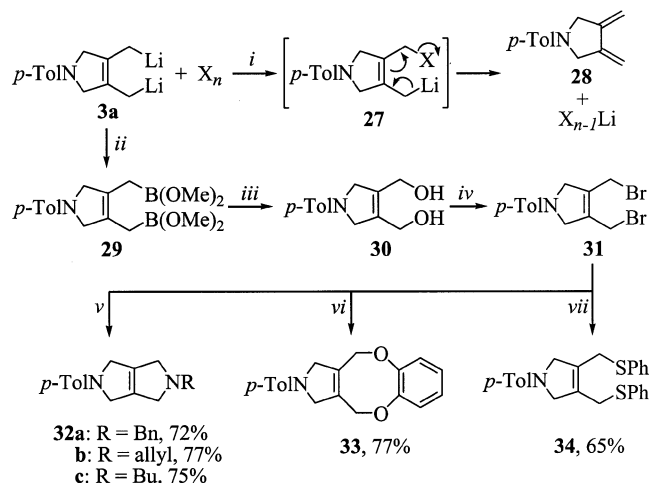
Scheme 6. Transformation of dianion 3a into dibromide 31 and further functionalization with nucleophiles; synthesis of compounds 32–34 ; reagents and conditions: i ) Et 2 O, –78 to 20 °C; ii ) B(OMe) 3 (2 equiv.), Et 2 O, –78 to 20 °C; iii ) NaOH/H 2 O 2 (4 equiv.), 0 °C and then reflux, 30 min; iv ) HBr (48%); v ) RNH 2 (1 equiv.), K 2 CO 3 (2 equiv.), CH 3 CN, reflux; vi ) catechol (1 equiv.), K 2 CO 3 (2 equiv.), (CH 3 ) 2 CO, reflux; vii ) PhSH (2 equiv.), NaOH (0.7 M), H 2 O/THF, 20 °C.
