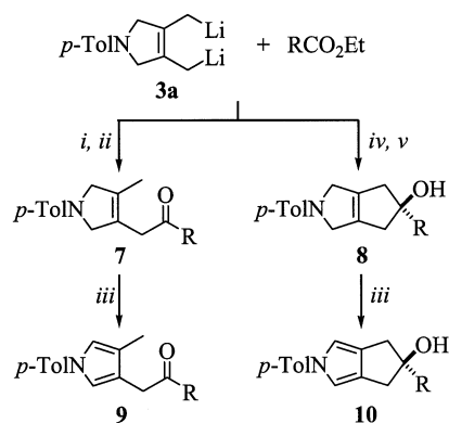
Scheme 2. Synthesis of functionalized pyrrole derivatives 7–10 ; reagents and conditions: i ) Et 2 O, –78 °C, 1 h; ii ) MeOH, –78 to 20 °C; iii ) DDQ (CH 2 Cl 2 , 1 equiv., 15 min) or air (CH 2 Cl 2 , 24 h); iv ) Et 2 O, –78 to 20 °C, 12 h; v ) H 2 O, 20 °C
