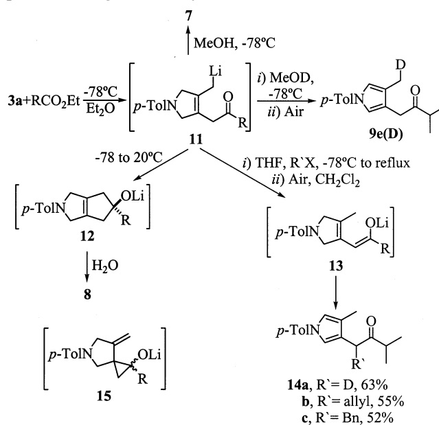
Scheme 3. Proposed mechanism for the selective formation of ketones 7 and alcohols 8
