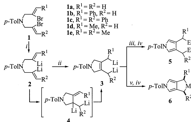
Scheme 1. Synthesis of functionalized pyrrole derivatives 5 and 6 ; reagents and conditions: i ) t BuLi (4 equiv.), \text{Et}_2\text{O} , -78\text{ }^{\circ}\text{C} ; ii ) TMEDA (4 equiv.), -78 to 20\text{ }^{\circ}\text{C} ; iii ) \text{E}^+ (2.2 equiv., see Table 1), -78 to 20\text{ }^{\circ}\text{C} ; iv ) DDQ ( \text{CH}_2\text{Cl}_2 , 1 equiv., 15 min); v ) \text{MCl}_2 (1 equiv.), -78 to 20\text{ }^{\circ}\text{C}
