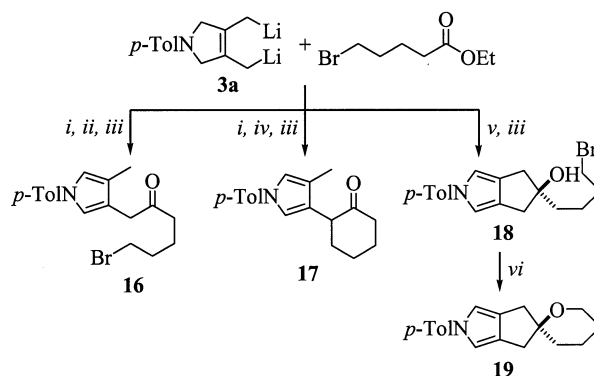
Scheme 4. Preparation of pyrroles 16–19 by treatment of 3a with ethyl 5-bromovalerate; reagents and conditions: i) \text{Et}_2\text{O} , -78^{\circ}\text{C} , 1 h; ii) \text{MeOH} , -78 to 20^{\circ}\text{C} ; iii) air ( \text{CH}_2\text{Cl}_2 , 24 h); iv) THF, -78 to 20^{\circ}\text{C} ; v) \text{Et}_2\text{O} , -78 to 20^{\circ}\text{C} , 12 h; vi) NaH (1.5 equiv.), THF, reflux, 24 h.
